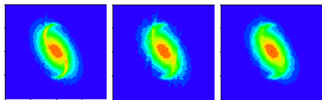
Figure 2. Y-Y' plane tomographic recovery of the phantom phase space distribution using different numbers of "measured" and interpolated projections. From left to right: a. 32 projections, b. 16 projections, c. 16 projections and 16 interpolations.
