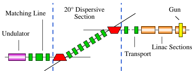
Figure 3: VISA beam line layout at ATF.
