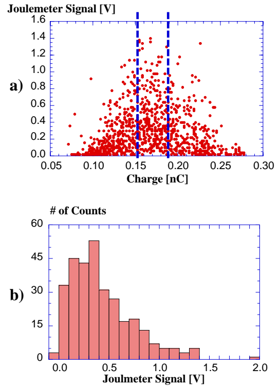
Figure 4: (a) FEL pulse energy measured with respect to the charge for 1500 consecutive shots at pop-in 8; (b) statistical distribution of the pulse energies within the 20% charge cut window.
